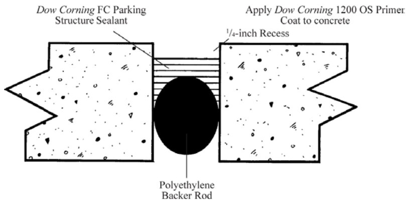
Figure 1: Good Joint Design
